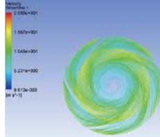
CFD flow field simulation diagram
