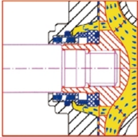
Single-end mechanical seal
