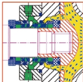
Double-end mechanical seal
