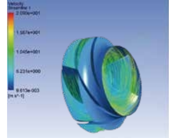
CFD flow field simulation diagram
